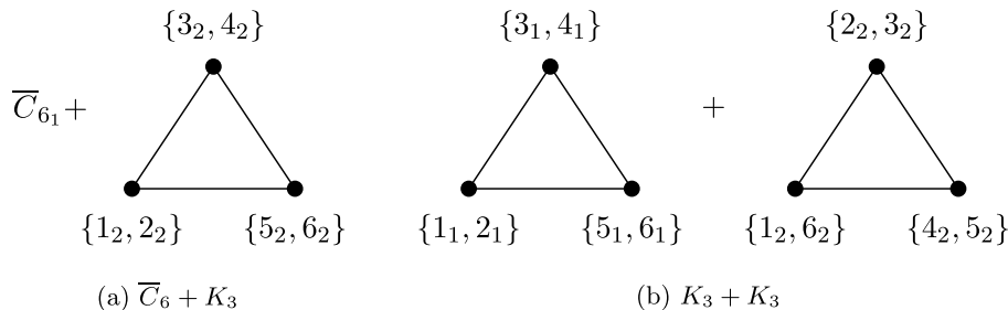
FIGURE 3. \overline{C}_6 + K_3 and K_3 + K_3
